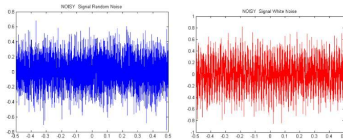
Fig.4.1 Random & White Noise
